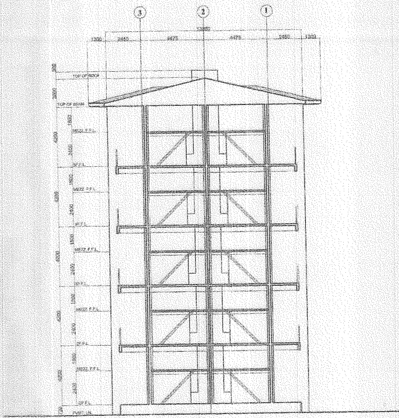
CROSS SECTION (C)
