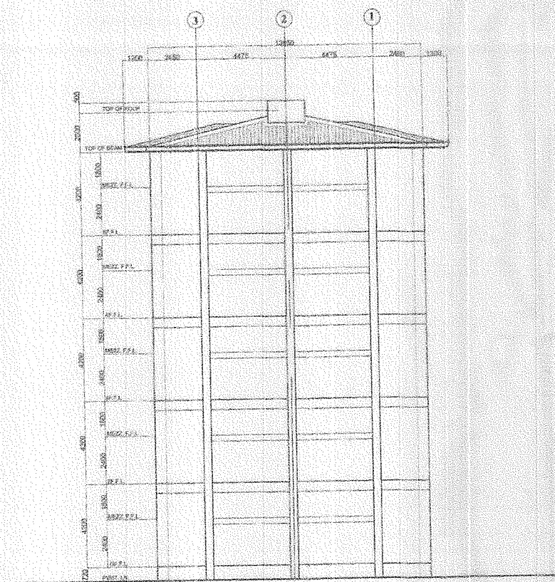
TYP. LEFT & RIGHT SIDE ELEVATION
